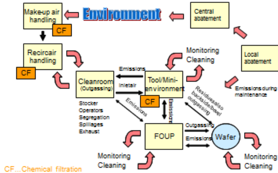
Figure FAC5 Total AMC concept
