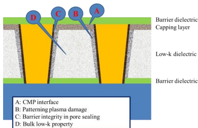
Figure MM-10 Degradation paths in low- \kappa damascene structure
