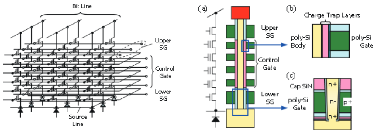
Figure MM-11 (left) A 3D NAND array based on a vertical channel architecture. (right) BiCS (bit cost scalable) – a 3D NAND structure using a punch and plug process [41].
