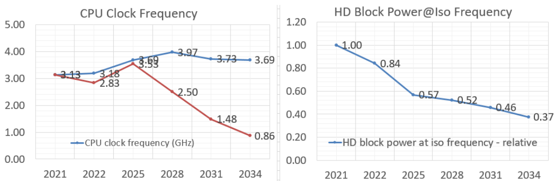
Figure MM-8 CPU clock frequency and power@iso-frequency (ref: 2021) scaling
