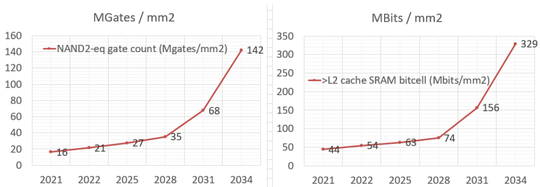
Figure MM-7 NAND2-equivalent standard cell count (left) and 111-bitcell (right) scaling in an 80\text{mm}^2 die
