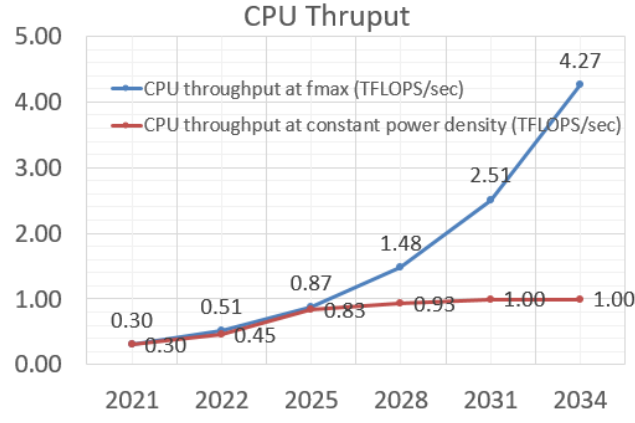
Figure MM-9 Scaling projection of computation throughput of CPU cores at the maximum clock frequency and at thermally constrained average frequency
