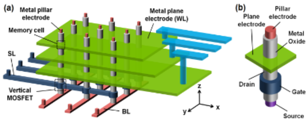
Figure MM-12 Schematic view of (a) 3D cross-point architecture using a vertical RRAM cell and (b) a vertical MOSFET transistor as the bit-line selector to enable the random access capability of individual cells in the array [52].
